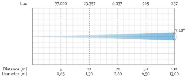
GOLUX 1000 | BEAM ANGLE 7,40°
